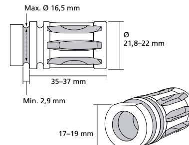
Required dimensions of NATO A1/A2 flash hiders for QM2.
